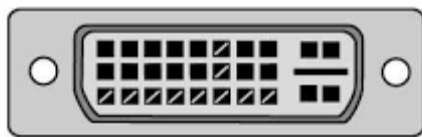
Dual Link DVI-I
